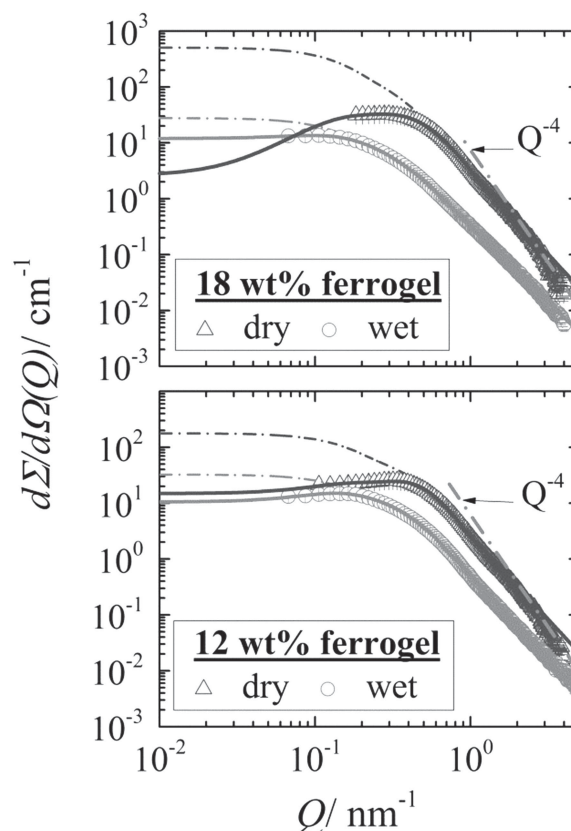
Figure 6. SAXS intensity d\Sigma/d\Omega(Q) versus scattering vector Q for a 18 and 12 wt% wet and dry ferrogel. In all cases the structure factor S(Q) was not negligible. Therefore, the data were fitted with the product of Equation S2 in the SI (structure factor) and the Beaucage equation (form factor) as shown by the solid lines. The dashed dotted lines represent the form factor of the particles.
