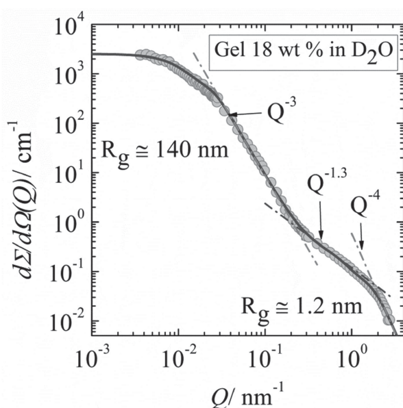
Figure 1. SANS macroscopic cross-section d\Sigma/d\Omega versus scattering vector Q for 18 wt% gelatin in \text{D}_2\text{O} ( T = 20^\circ\text{C} ). At low Q ( < 0.02 \text{ nm}^{-1} ) USANS data are also presented after rescaling. The solid line represents a fit of the two levels Beaucage equation.
